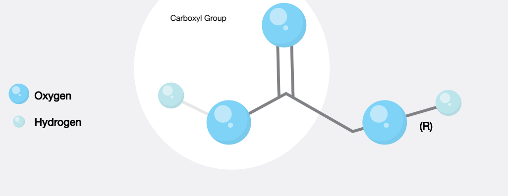
Figure 1 The Molecular Structure of Glycolic Acid
